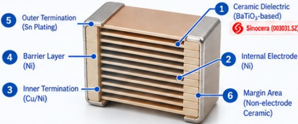
MLCC STRUCTURE (3D CUTAWAY)
