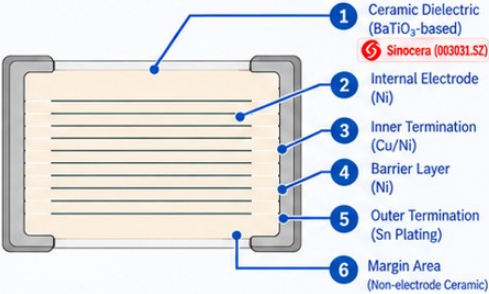
MLCC STRUCTURE (CROSS-SECTION)
